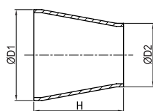
MANUAL WELDING TYPE (125A ~ 200A)
