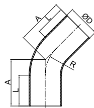
AUTO WELDING 45° ELBOW (8A~100A) (1/4"~6")
