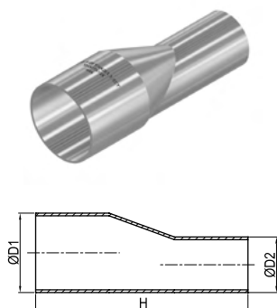
AUTO WELDING TYPE (8A~100A)
